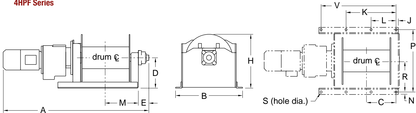
4HPF Series Winch Dimensions
